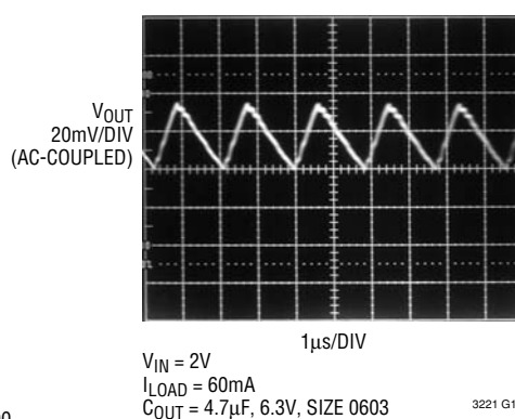
Output Ripple
